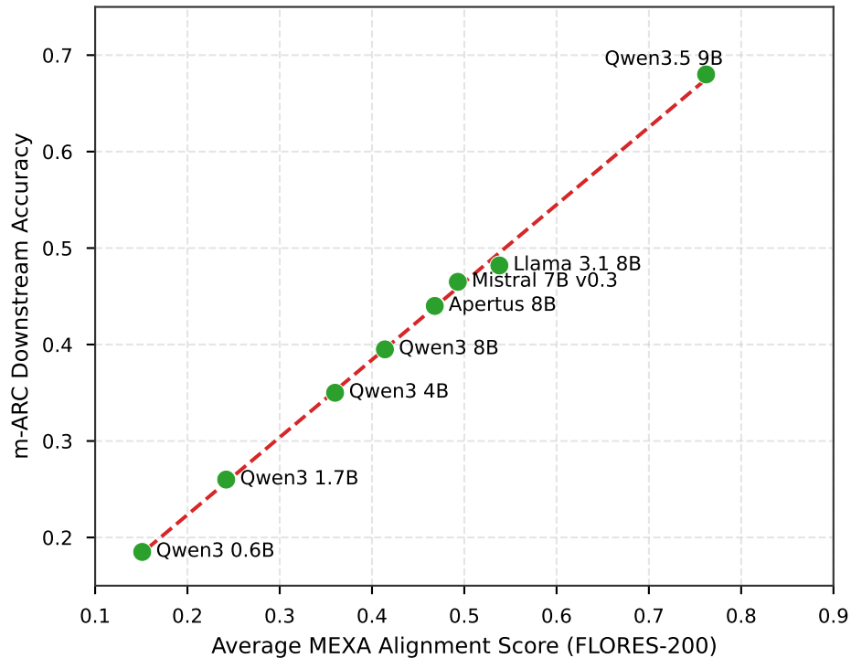
MEXA vs. m-ARC Accuracy (Spearman \rho = 1.000 )
